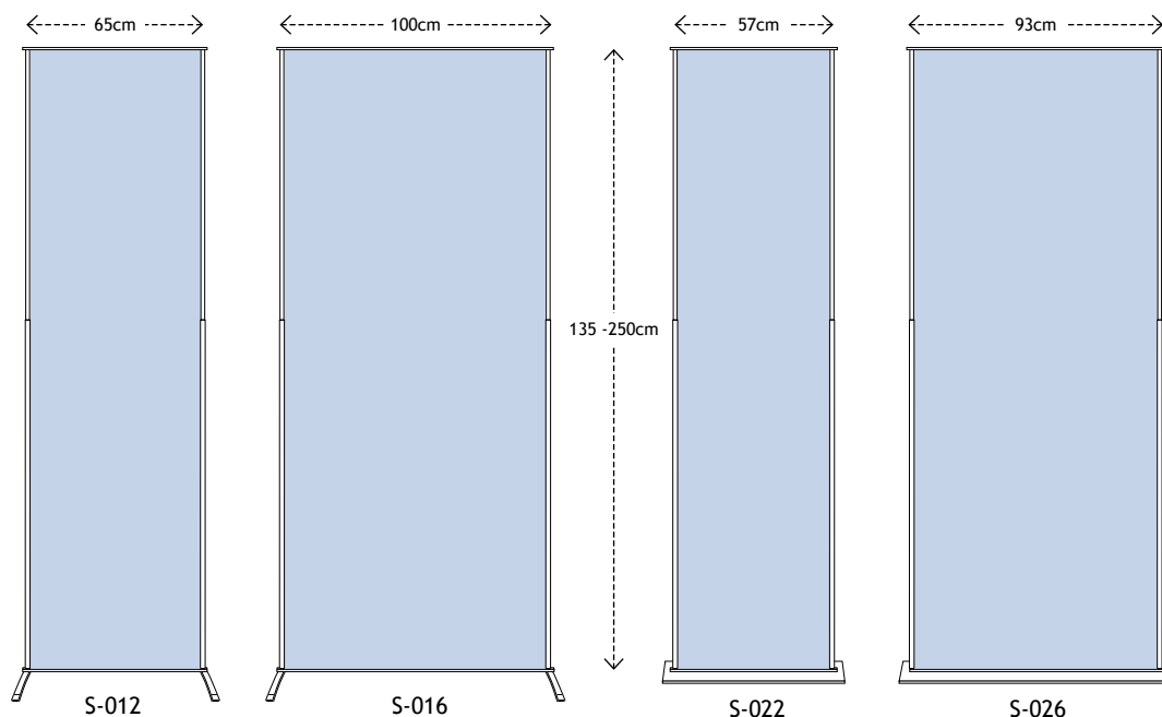
FLEX-display™ Frame, with base plate
